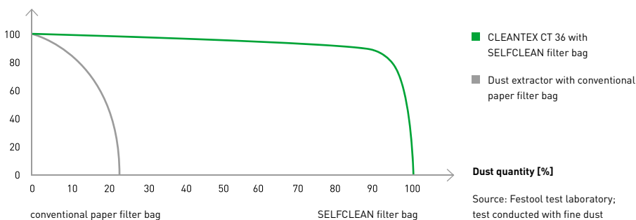
Suction power [%]
