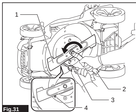
Fig.31 ► 1. Mower blade 2. Wrench 3. Screwdriver 4. Hole
